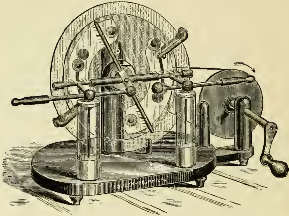
TOEPLER-HOLTZ ELECTRICAL MACHINE.
